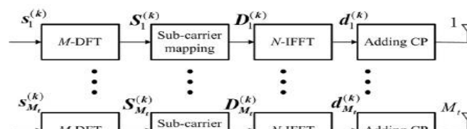
Fig. 1. MIMO SC-FDMA transmitter for user k with M_t transmit antennae.
